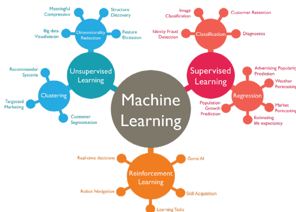
Figure 2: Machine learning
